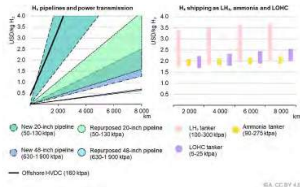
Figure 5.13: Cost comparison of hydrogen transport options (USD/kg) (source: IEA, 2023)
